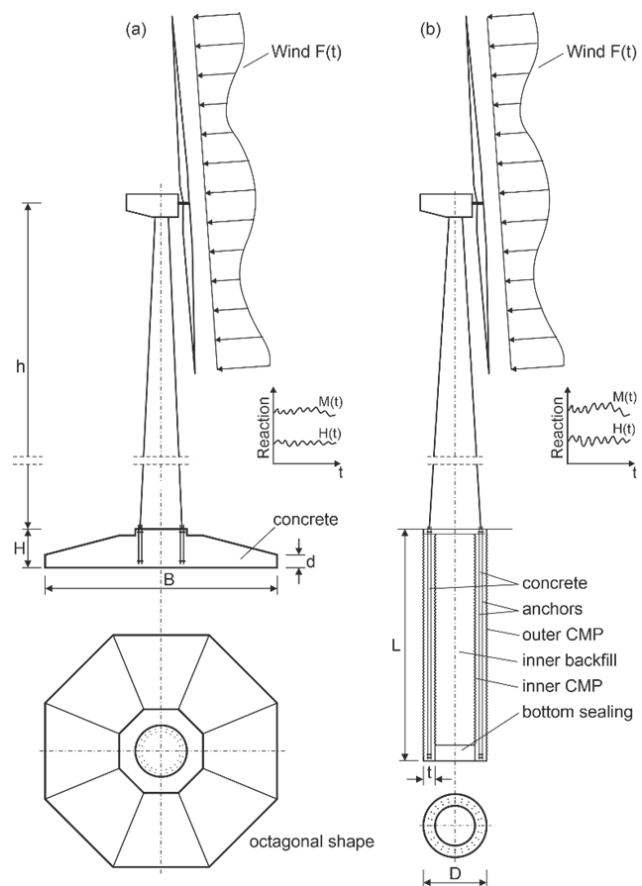
Fig. 1 Schematic sketch of shallow foundation (a) and pier foundation (b)
