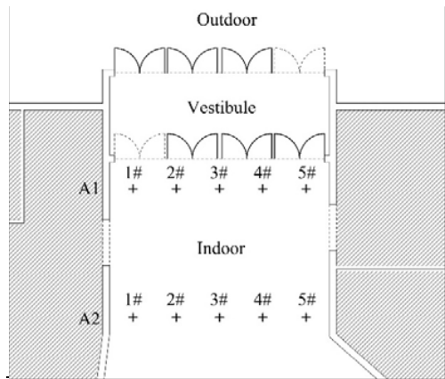
Fig. 6 Measuring points
