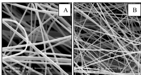
Fig. 10 SEM Images of Electrospun PAN nanofibers (A) at 2000X resolution and (B) at 1200X resolution using rotating drum collector
