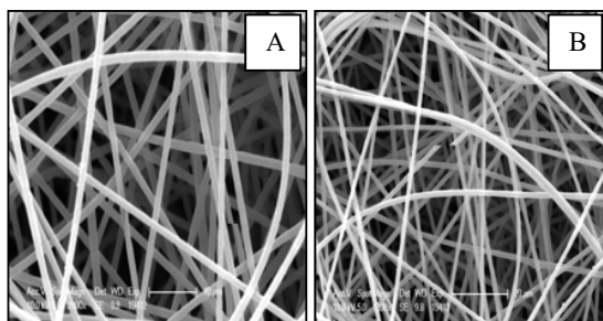
Fig. 10 SEM Images of Electrospun PAN nanofibers (A) at 2000X resolution and (B) at 1200X resolution using Flat plate collector
