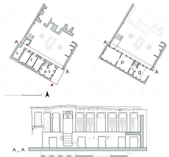
Fig. 3 Nili's House: floor plans and façade, p: principal chamber, s: storage, g: guest room, i: Iwan , r: resting room
