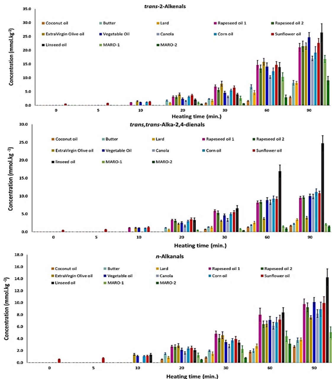
Fig. 2 Bar diagram plots of the mean \pm SEM ^1\text{H} NMR-determined concentrations of trans -2-alkenals (top), trans,trans -alka-2,4-dienals (middle) and n -alkanals (bottom) in mmol.kg ^{-1} units in a wide series of culinary oils, butter and lard samples when exposed to laboratory-simulated shallow-frying episodes for periods of 0, 5, 10, 20, 30 60 and 90 min. A colour key is provided for each frying medium (frying oils, butter or lard) tested in this manner. Abbreviations: MARO-1 and -2 (light- and dark-green colour codes respectively) represent MUFA (oleoylglycerol)-rich algae frying oils
