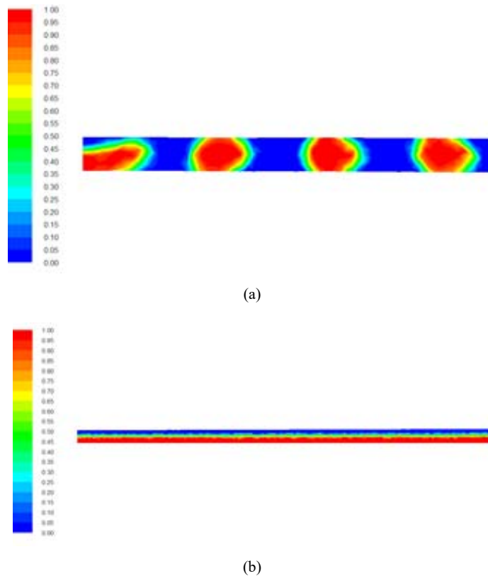
Fig. 2 Effect of Q_{aq} on HD flow regime in mixing channel at vertical slice ( y=0 ), (a) R=1 , Q_{or}=2 mL/min, (b) R=1 , Q_{or}=6 mL/min
