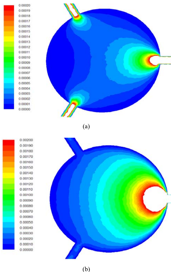
Fig. 5 CFD results of the velocity contour in a horizontal shear ( y = 0 ) in the micromixer in the absence of and presence of ultrasonic waves, R=1 , Q_{or}=6 mL/min. (a) absence of ultrasound, (b) presence of ultrasound
