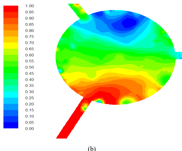
Fig. 4 CFD results of the flow regime in a horizontal shear ( y = 0 ) in the micromixer in the absence of and presence of ultrasonic waves, R=1 , Q_{or}=6 mL/min. (a) absence of ultrasound, (b) presence of ultrasound
