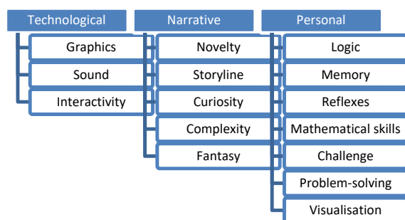
Fig. 4 GBL attributes [15], [16]
