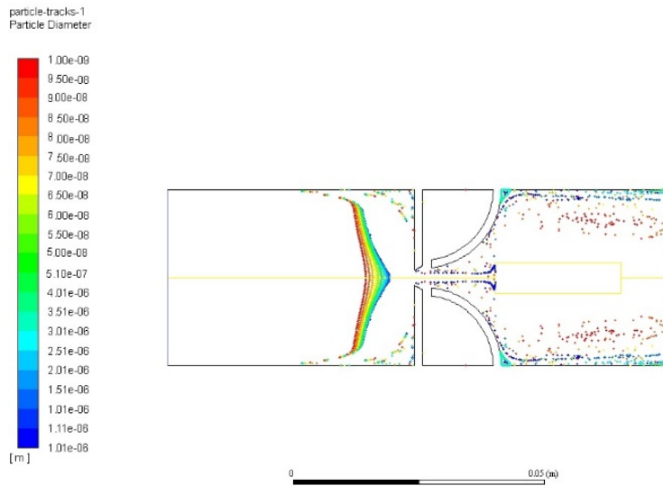
Fig. 8 Particle diameter
