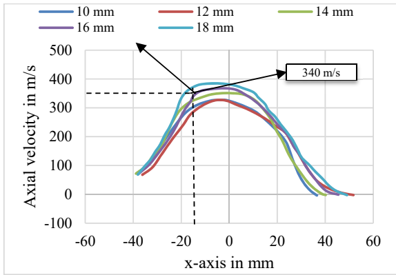
Fig. 5 The axial velocity along the x-axis with the length of the section between the lens (x = 0) and FCE being x = (10 mm, 12 mm, 14 mm, 16 mm and 18 mm)
