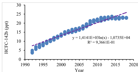
Fig. 3 Logarithmic adjustment
