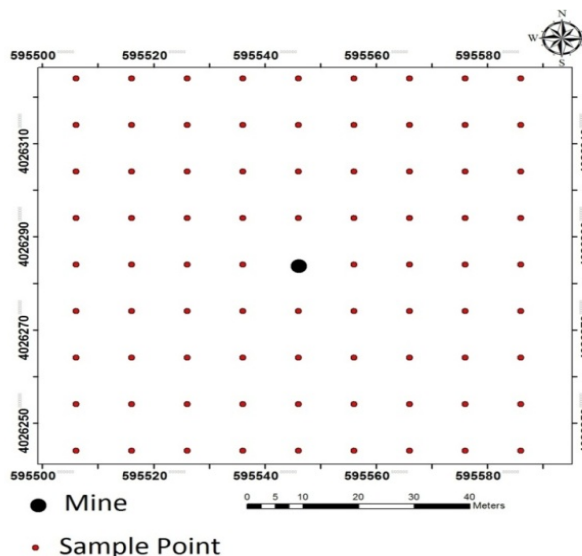
Fig. 2 Sample points in order to consider spatial changes in soil properties
