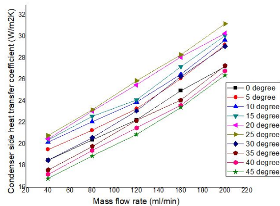
Fig. 6 Comparisons of condenser heat transfer coefficient with mass flow rate at different angle of inclination
