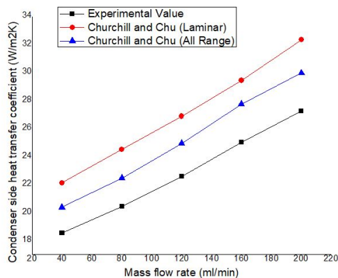
Fig. 5 Variation of condenser heat transfer coefficient with mass flow rate at 0° inclination
