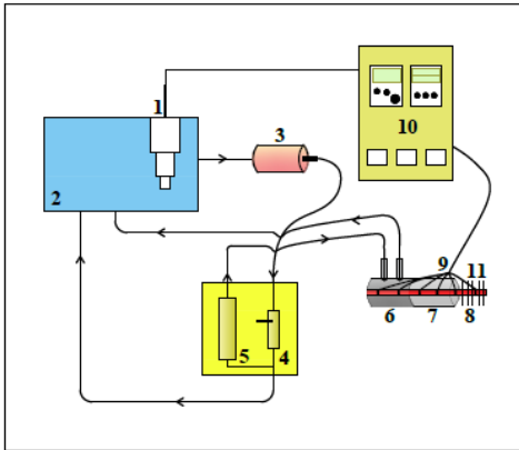
Fig. 1 Schematic heat pipe with annular fins test rig used in this study
