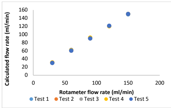
Fig. 3 Calibration of rotameter
