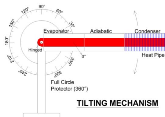
Fig. 2 Schematic diagram of tilting mechanism
