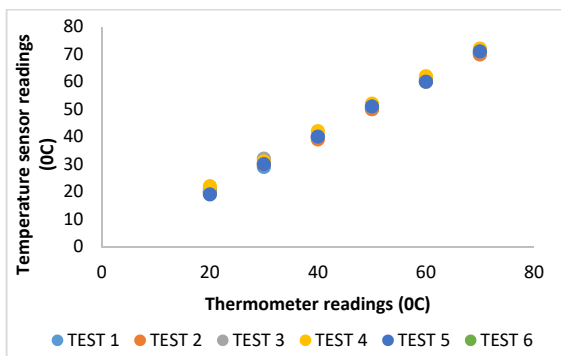
Fig. 4 Calibration of temperature sensor
