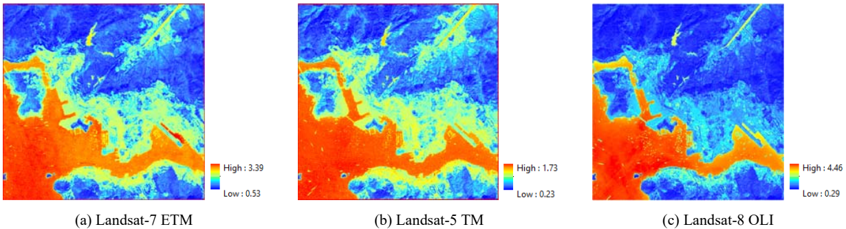
Fig. 4 Multi-temporal TCWVI maps
