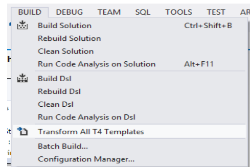
Fig. 5 Template Transformation
