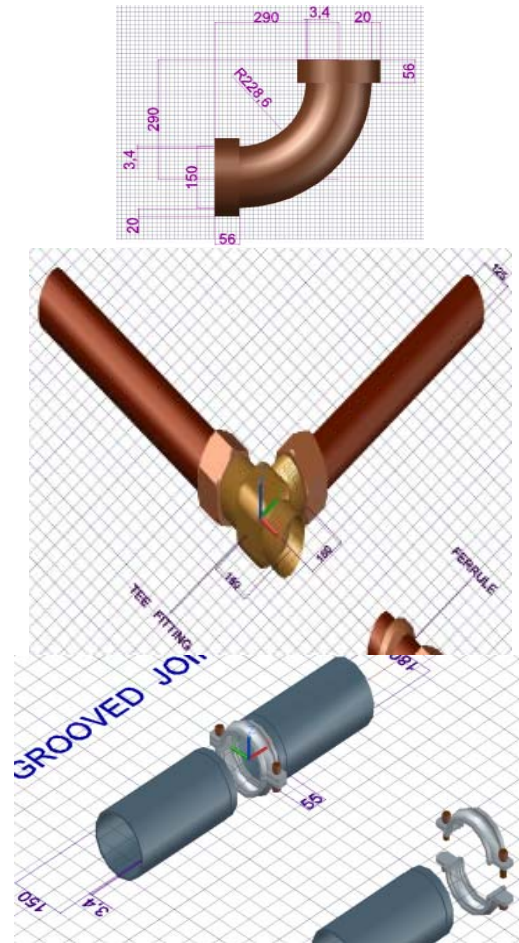
Fig. 1 Pipeline Model
