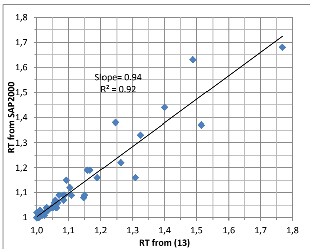
Fig. 11 Comparison between period ratio (RT) from both SAP2000 and (13) for data used in derived equation
