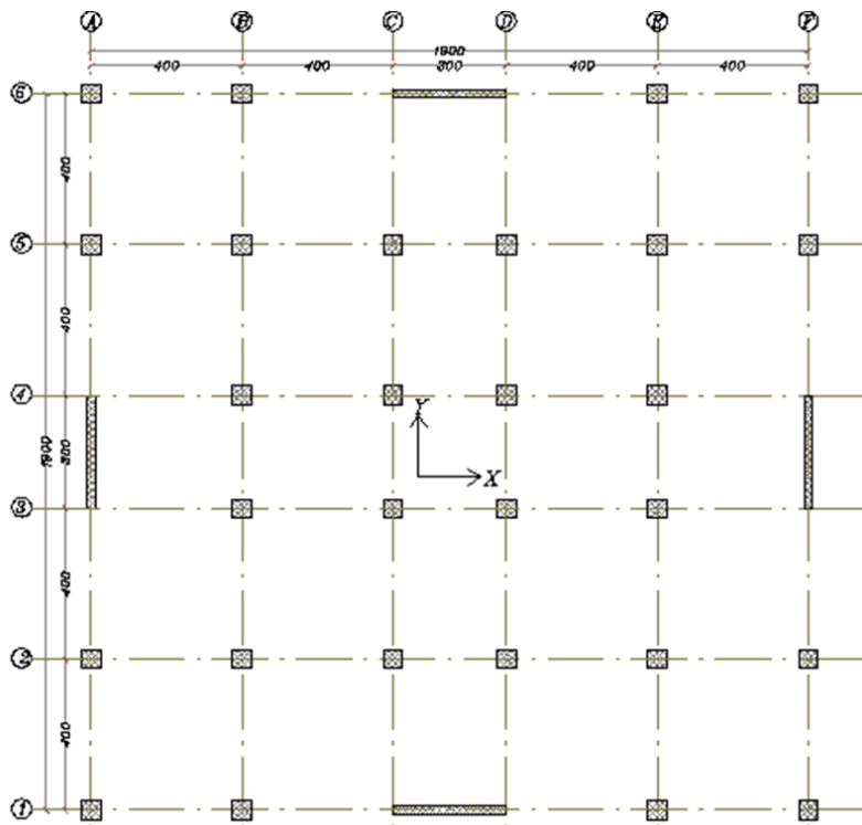
Fig. 2 Second building layout
