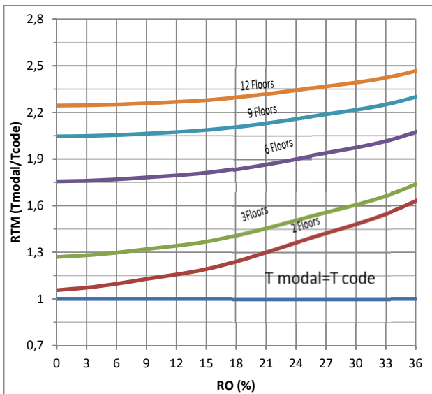
Fig. 9 Opening ratio versus period ratio ( T_{modal}/T_{code} ) for different number of building height for the first building layout using detailed code formula
