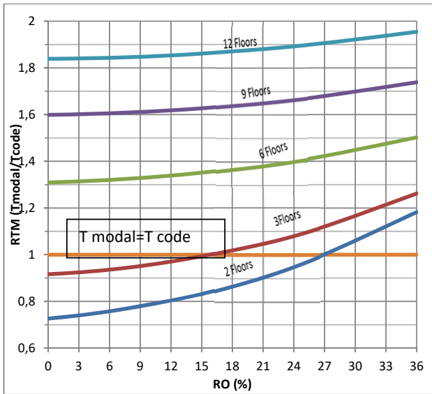
Fig. 8 Opening ratio versus period ratio ( T_{modal}/T_{code} ) for different number of building height for the second building layout using general code formula
