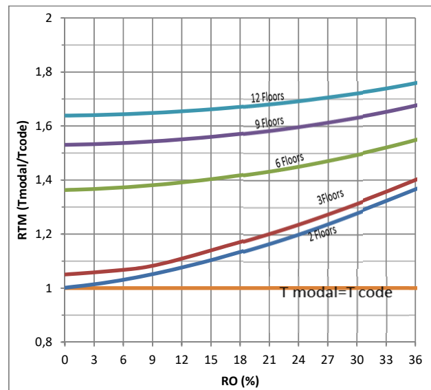
Fig. 10 Opening ratio versus period ratio ( T_{modal} / T_{code} ) for different number of building height for the second building layout using detailed code formula
