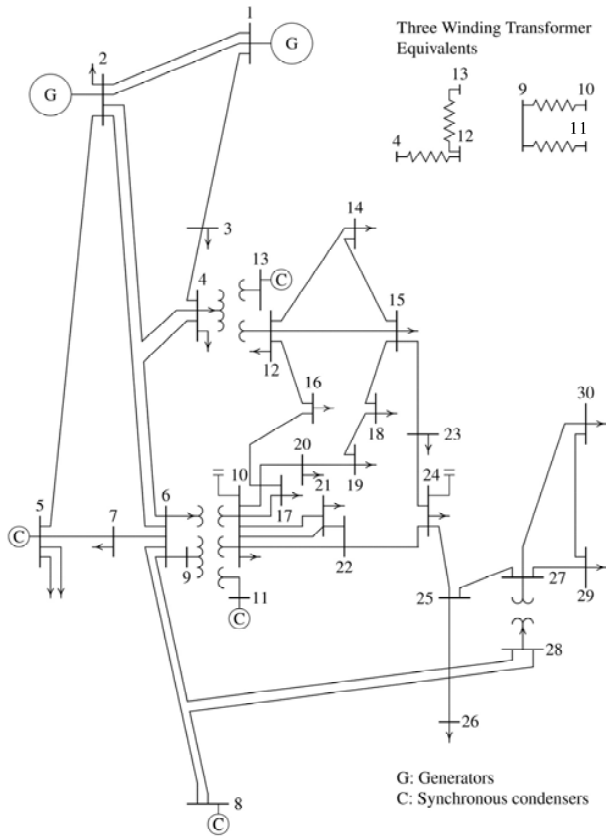
Fig. 1 IEEE 30 Bus Test System
