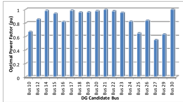
Fig. 3 Optimal Power Factor for DG at Allied Bus
