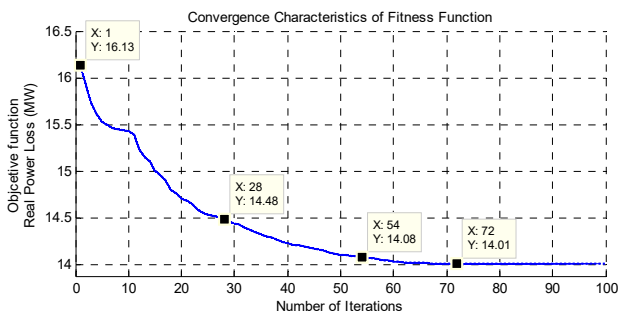
Fig. 5 Convergence Characteristics of PSO Algorithm for Optimal DG Placement @ Bus 21
