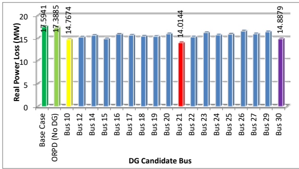
Fig. 4 Total Power Loss of Test System with and without DG Integrated at Allied Bus
