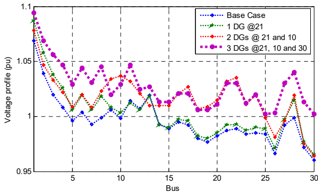
Fig. 6 System Voltages of Test System: Before and After DG
