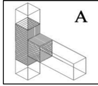
Fig. 11 FRP used to strengthening all around joint
