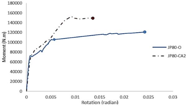
Fig. 12 Moment-rotation diagram for CA2 mode
