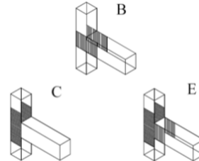
Fig. 5 Studied modes for shear strengthening
