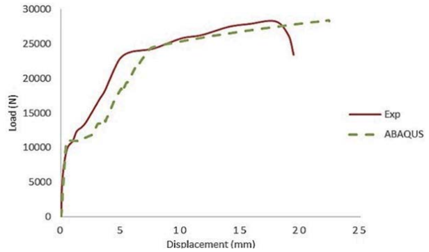
Fig. 3 FEM analyze and experimental results
