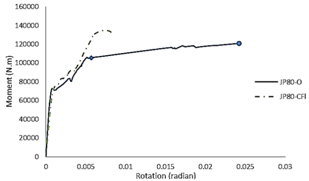
Fig. 10 Moment-rotation diagram for flexural strengthened joint
