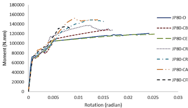
Fig. 15 Moment-rotation diagram for CA2 mode
