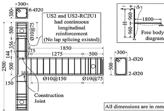
Fig. 1 Detail of base model joint
