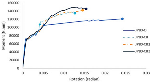
Fig. 8 Shear strengthening using 1- and 2-layer of FRP
