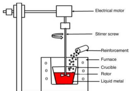
Fig. 1 Stir casting [5]
