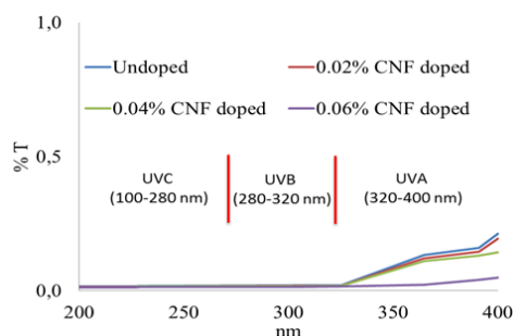
Fig. 9% Transmittances of samples
