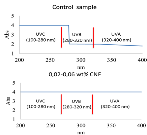
Fig. 8 UV absorbability of the control sample and sample with 0,02-0,06 wt% CNF
