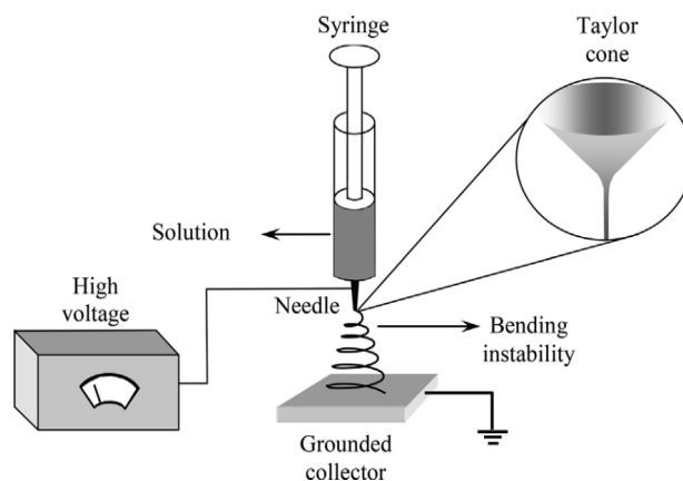
Fig. 2 Electrospinning setup [13]
