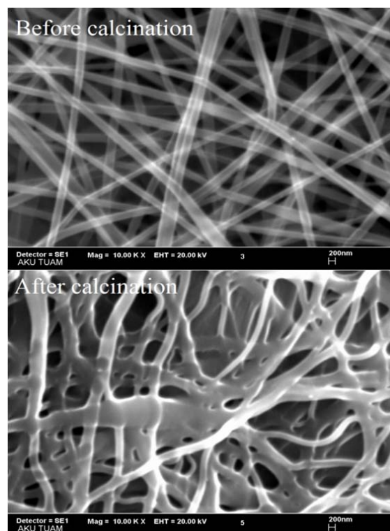
Fig. 3 SEM images of carbon nanofibers before and after calcination
