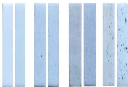
Fig. 5 CNF/RTV664 polymer composites (0-0,02-0,04-0,06% respectively)
