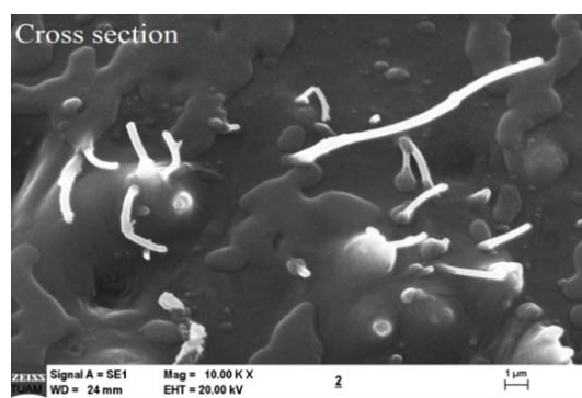
Fig. 7 SEM image of composite cross section
