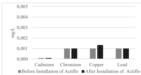
Fig. 17 Average concentration of Cadmium, Chromium, Copper and Lead in RO feed Water for the entire evaluated period
