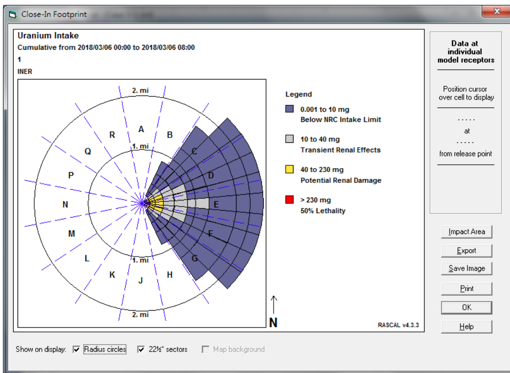
Fig. 6 The UF6 analysis result for Uranium intake
