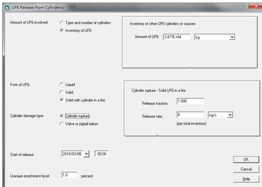
Fig. 2 The RASCAL setting for UF 6 analysis
