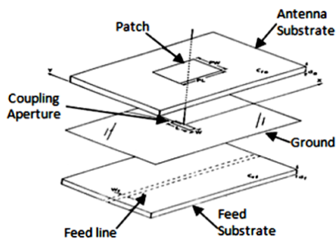
Fig. 17 Aperture coupled feed structure
