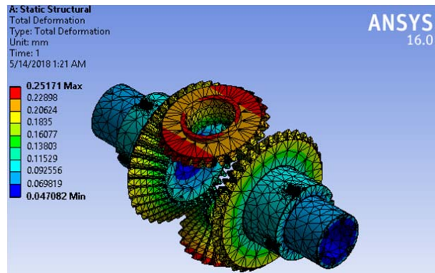
Fig. 7 Total deformation
