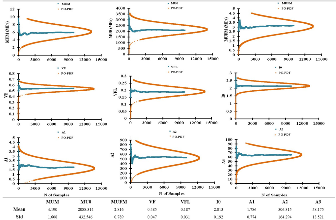
Fig. 2 Posterior probability distribution function (PO-PDF) and mean of calibrated material parameters (Bayesian calibration with 10000 MCMC). \mu_m (MUM) Shear modulus of the ligament matrix, \mu_0 (MU0) Shear modulus of the fibril, \mu_{fm} (MUFM) Shear modulus of the fiber matrix, v_f Volume fraction of the fibre, v_{fl} Volume fraction of the fibril, I_0 Secondary stiffening of the fibril, a_i Dimensionless fibril parameters
