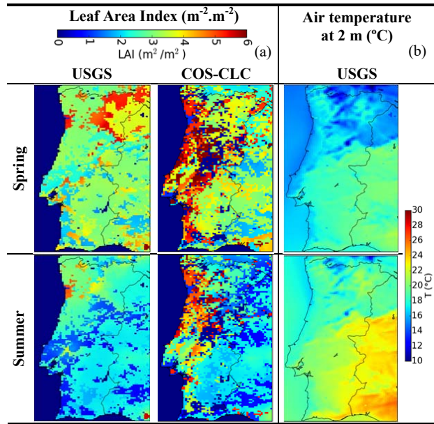
Fig. 4 (a) Average Leaf Area Index ( m^2.m^{-2} ) for the spring and summer using both LC approaches; (b) 2 m average air temperature ( ^{\circ}C ) for the spring and summer using the USGS LC approach
