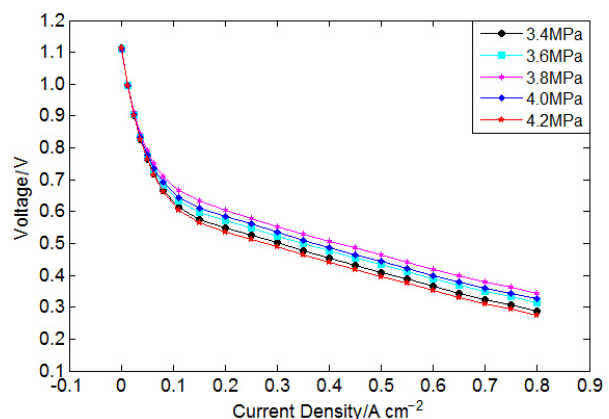
Fig. 12 Polarization curves under different locking pressure
