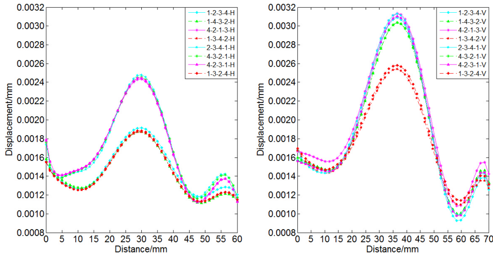
(a)The displacement of Z direction along H path (b)The displacement of Z direction along V path
