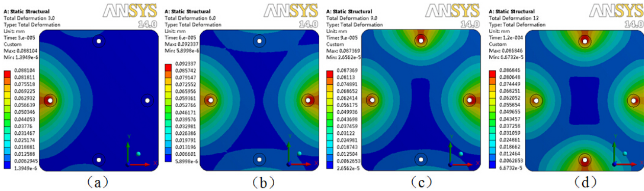
(a) Locking the first bolt (b) Locking the second bolt (c) Locking the third bolt (d) Locking the fourth bolt
