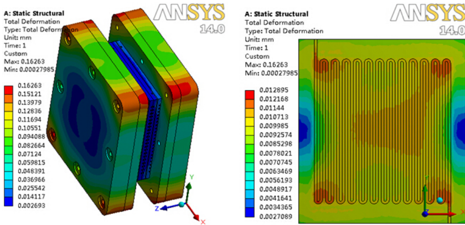
(a) The overall displacement contour
