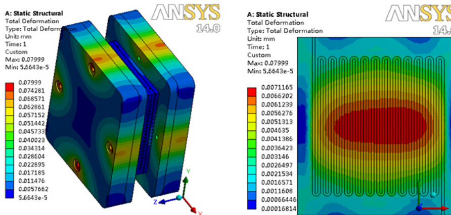
(a) The overall displacement contour
