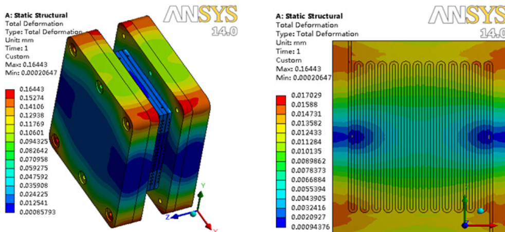
(a) The overall displacement contour
