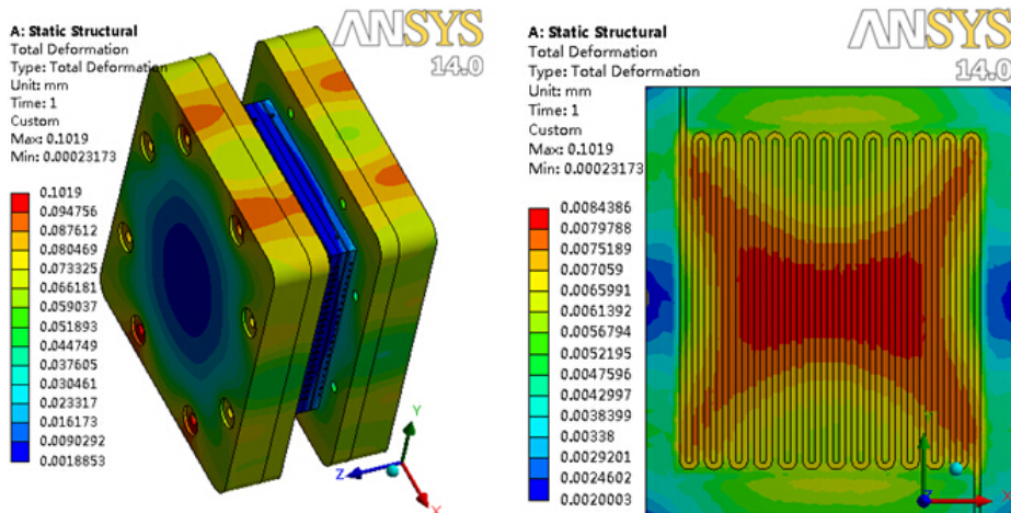
(a) The overall displacement contour
