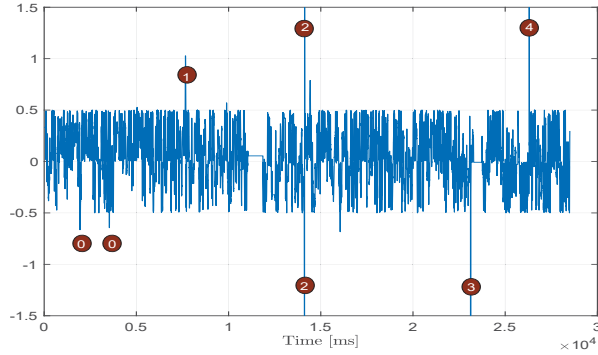
Fig. 9 Real-time lateral error sample data obtained during the 60km tour on M40 highwa- Madrid. The data demonstrating the undetectable lane marks on the road, cases 2,3, and 4
