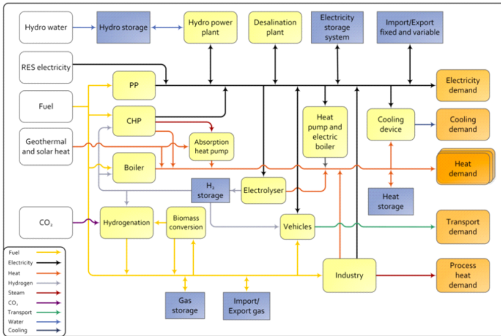
Fig. 4 Typical energy system in EnergyPLAN
