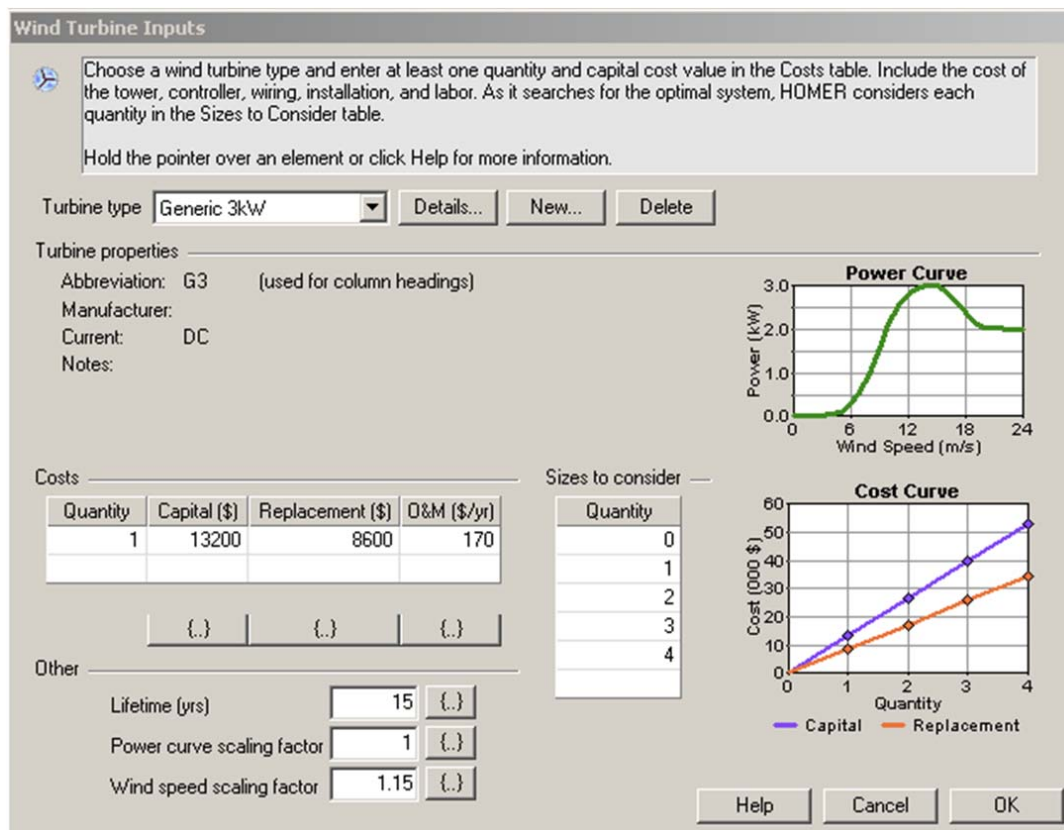
Fig. 1 HOMER's wind turbine inputs window [11]
