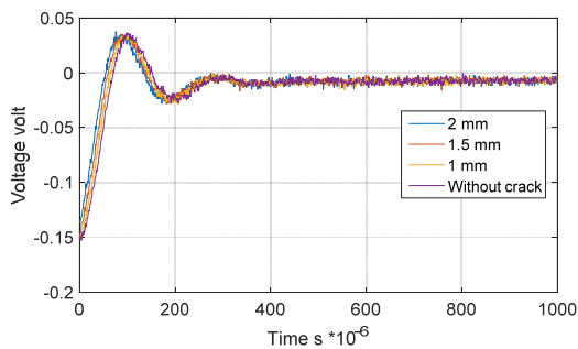
Fig. 5 PEC responses of three and without cracks
