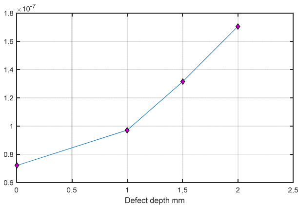
Fig. 9 Result of the pulse responses from the tree defects and without defects samples
