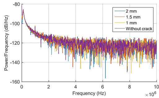
Fig. 6 PSD of PEC responses in Fig. 5
