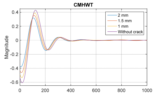
Fig. 7 CMHWT of PEC responses in Fig. 5
