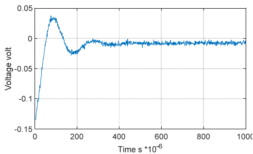
Fig. 4 PEC response from Aluminum sample
