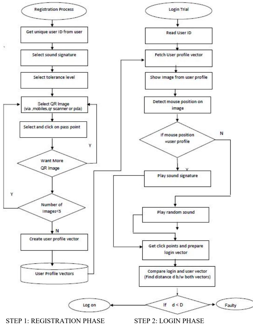
Fig. 3 Flowchart
