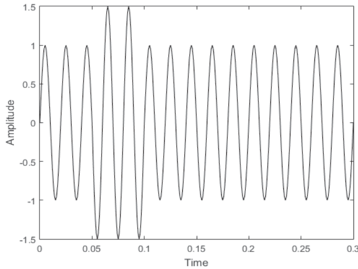
Fig. 3 Swell signal
