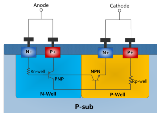
Fig. 1 The cross section view of conventional SCR
