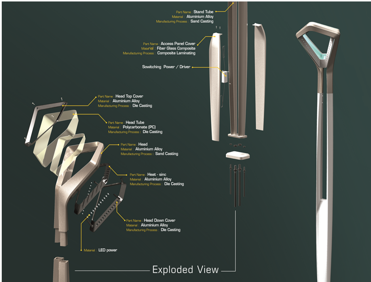
Fig. 11 Exploded view of smart urban lighting
