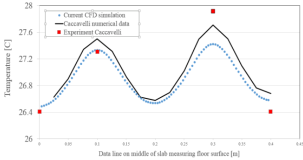
(a) Steady state heated floor validation
