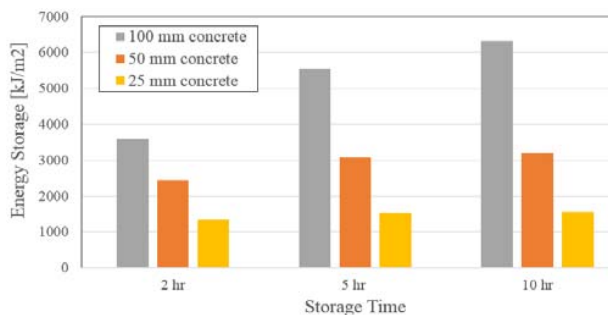
Fig. 9 Different concrete thickness heights energy stored
