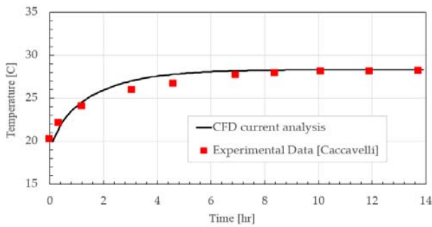
(b) Transient model validation, heating system active
