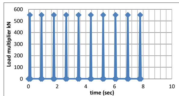
Fig. 6 Dynamic loading wave (speed = 40 km/h)
