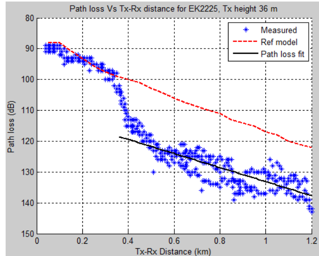
Fig. 6 A path loss curve for one of the urban environments (Maryhill, EK2225)
