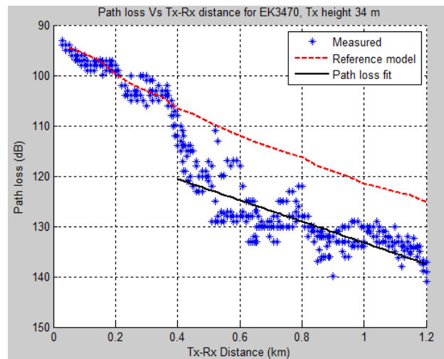
Fig. 7 A path loss curve for one of the suburban environments (Oye-Ekiti, EK3470)
