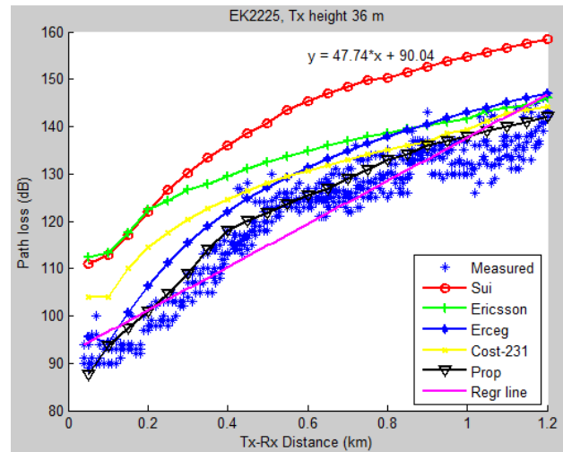
Fig. 8 Comparison of observed path losses in urban environment with proposed two slope, SUI, Ericson, Cost 231-Hata and Erceg models
