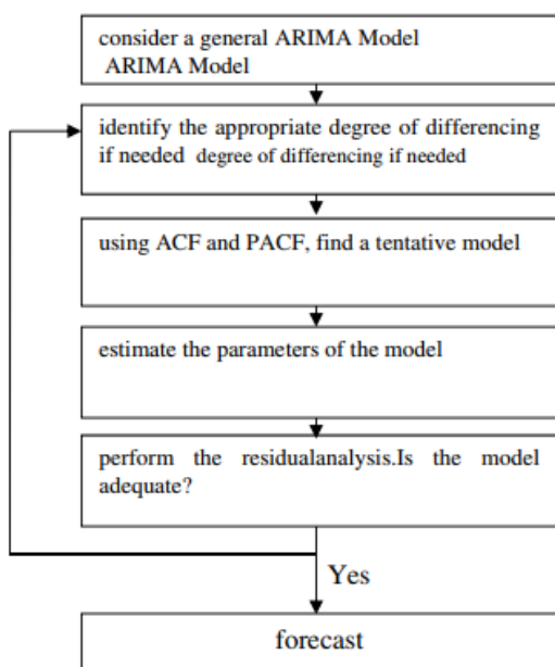
Fig. 2 ARIMA model development
