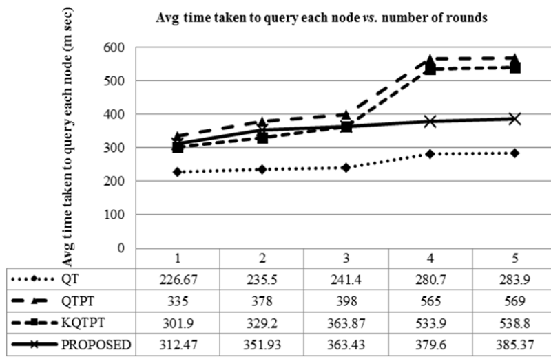
Fig. 12 Average of execution time at each node vs. number of rounds
