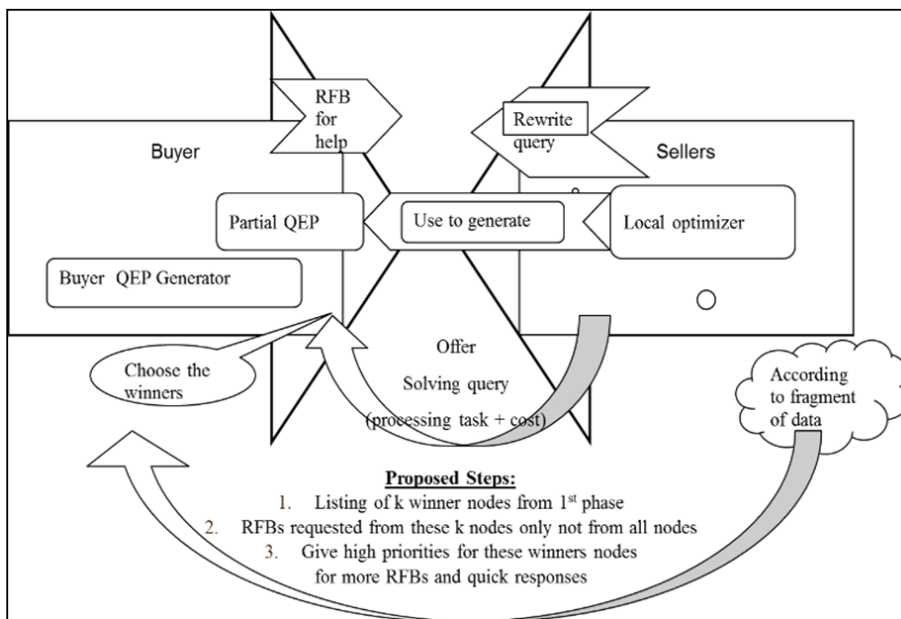
Fig. 7 Architecture of proposed strategy
