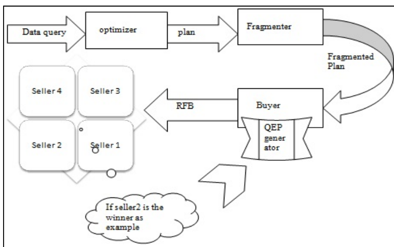
Fig. 3 Architecture of the Mariposa strategy
