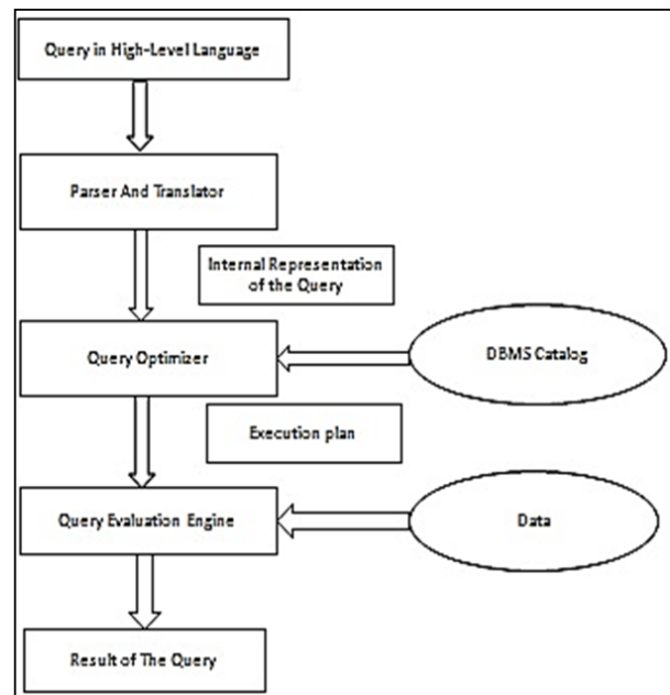
Fig. 1 Query processing steps
