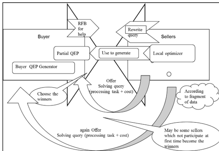
Fig. 5 Architecture of QTPT Strategy
