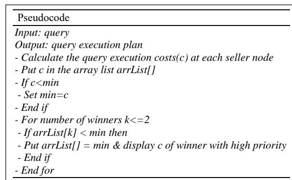
Fig. 9 Pseudocode of the proposed strategy
