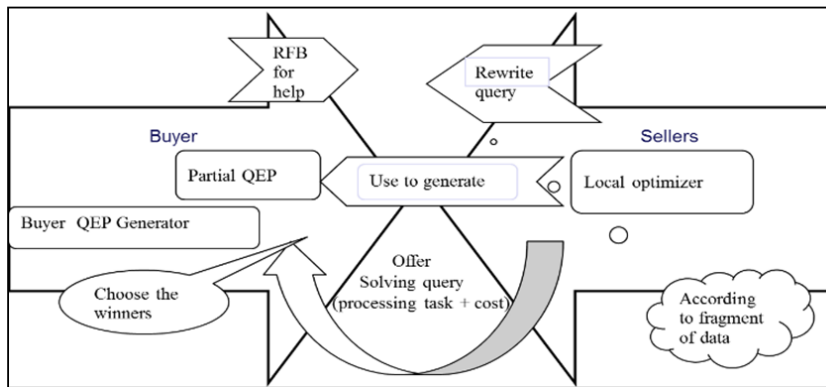
Fig. 4 Architecture of Query Trading
