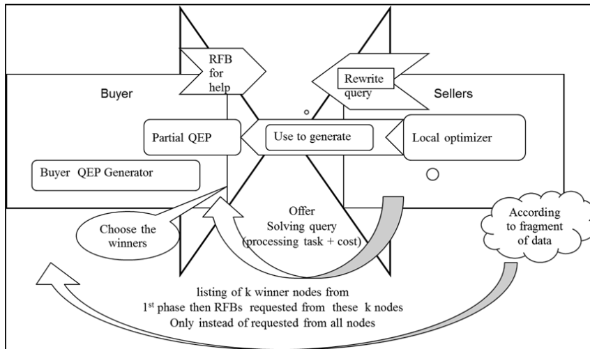
Fig. 6 Architecture of K-QTPT Strategy
