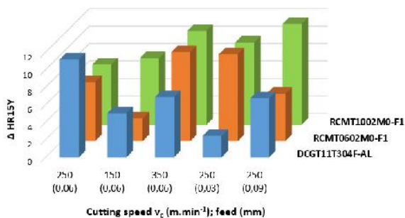
Fig. 5 Dependence of Tool Geometry and Cutting Conditions on \Delta HR15Y
