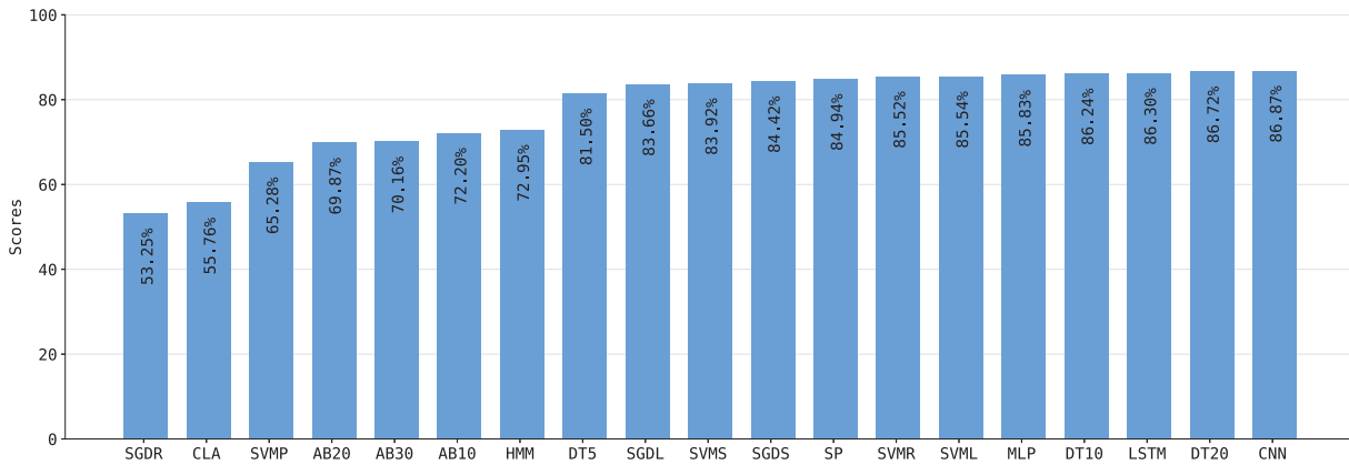
Fig. 1 The average F-measure score across all datasets
