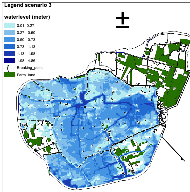
Fig. 6 Water depths for Pellworm Island under scenario 3
