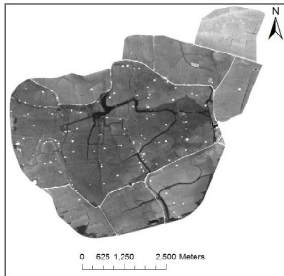
Fig. 4 Topography of Pellworm Island in ArcGIS
