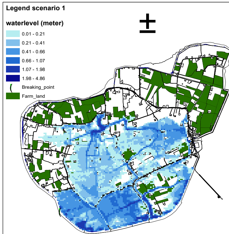
Fig. 5 Water depths for Pellworm Island under scenario 1
