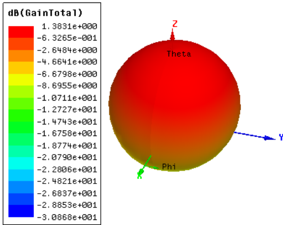
Fig. 11 Gain at 5.21 GHz
