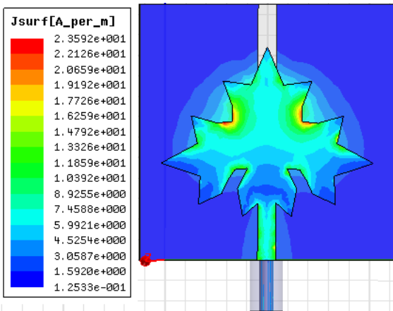
Fig. 8 Current Distribution at 5.21 GHz
