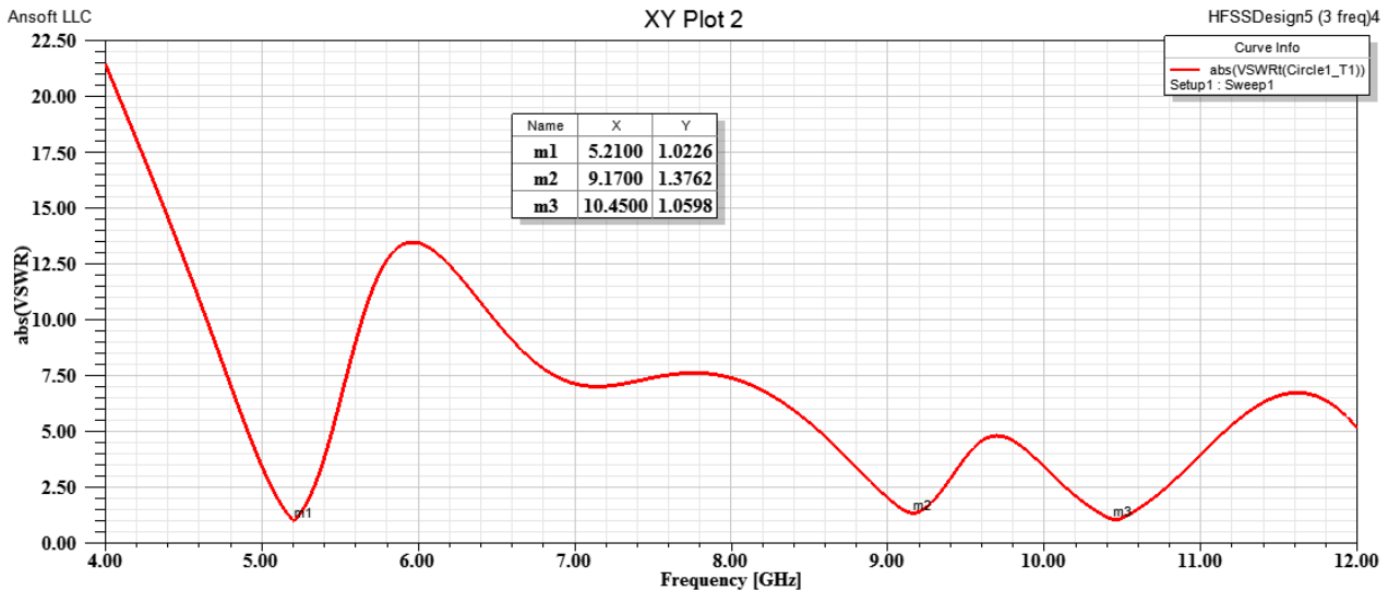
Fig. 14 VSWR plot for the proposed model
