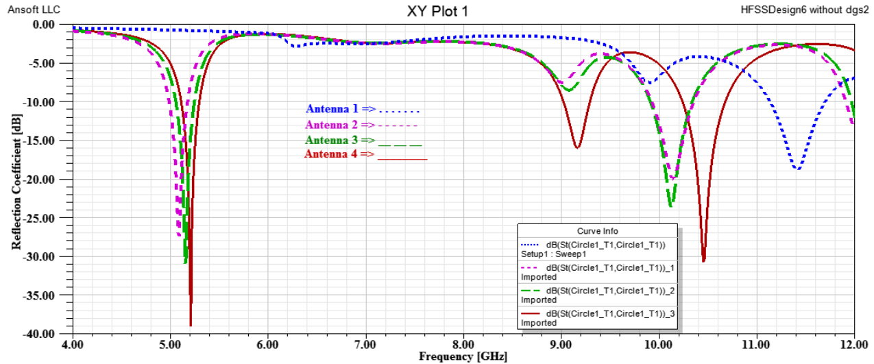
Fig. 5 Return loss comparison
