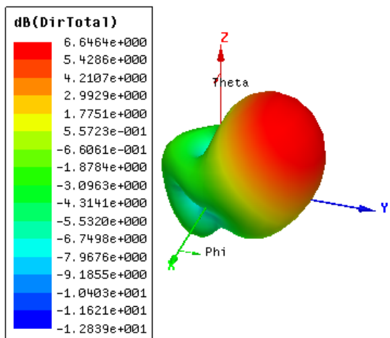
Fig. 16 Directivity at 9.17 GHz
