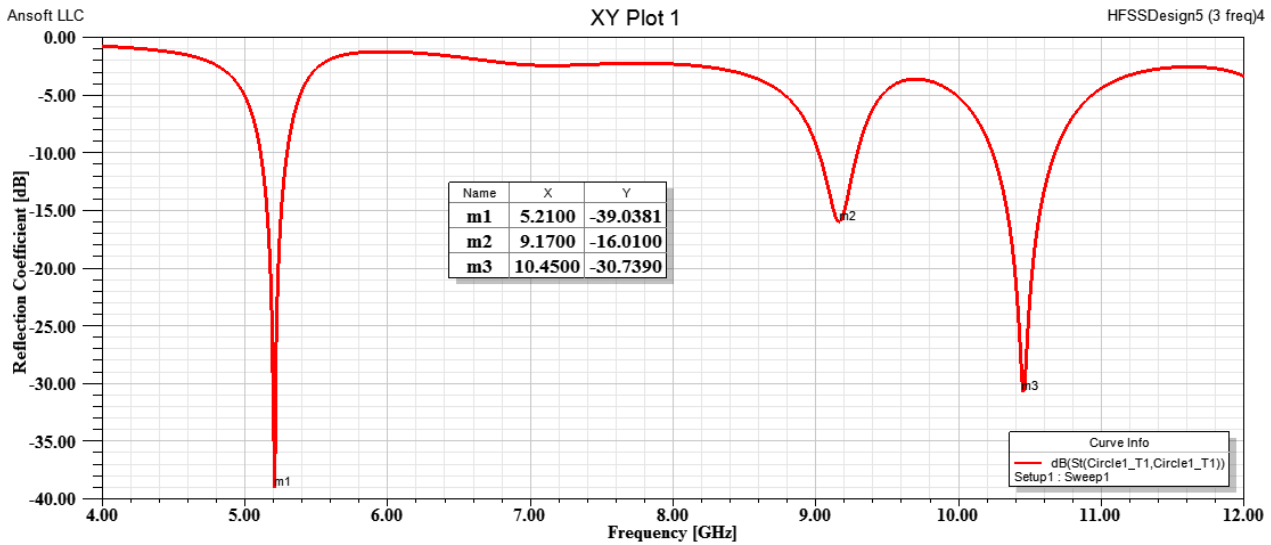
Fig. 7 S-parameter for the Proposed Model
