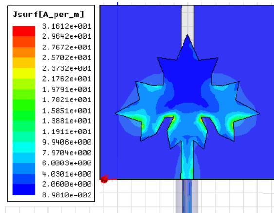
Fig. 10 Current Distribution at 10.45 GHz
