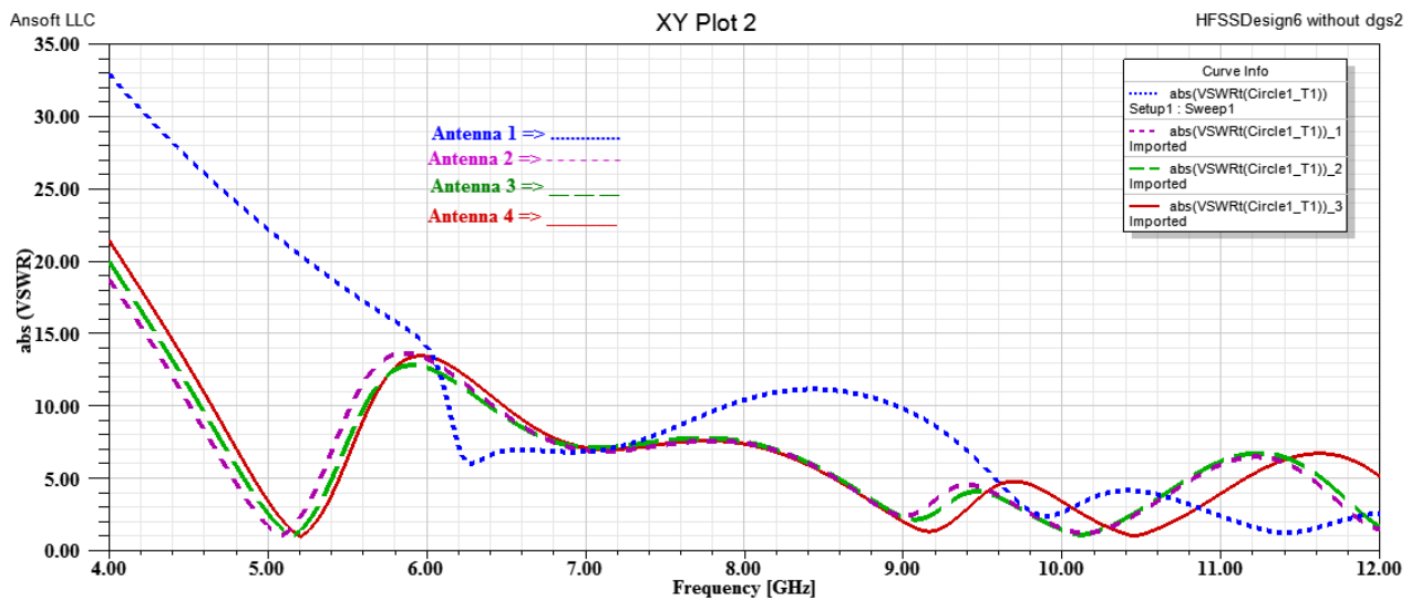
Fig. 6 VSWR comparison
