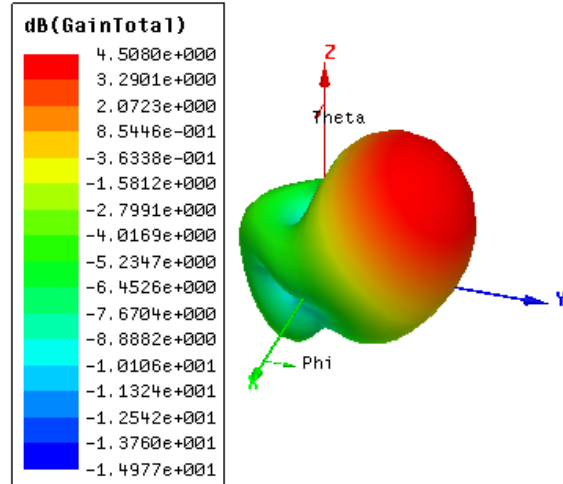
Fig. 12 Gain at 9.17 GHz
