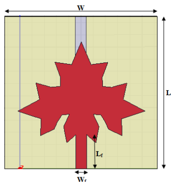
Fig. 2 Proposed Design Model – view at front
