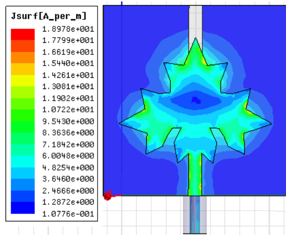
Fig. 9 Current Distribution at 9.17 GHz
