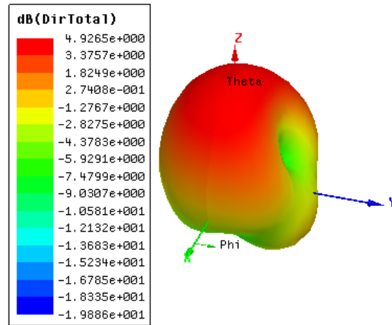
Fig. 17 Directivity at 10.45 GHz
