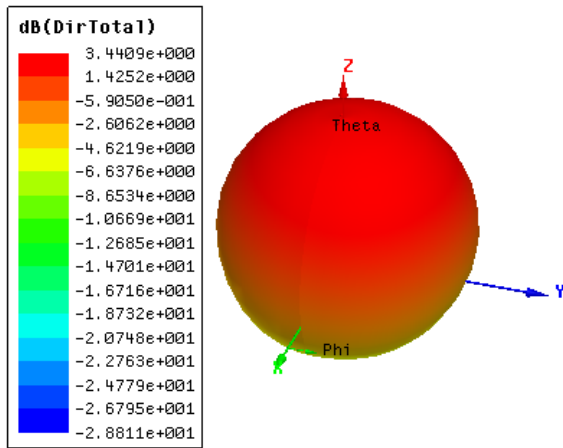
Fig. 15 Directivity at 5.21 GHz
