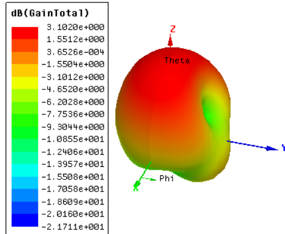
Fig. 13 Gain at 10.45 GHz
