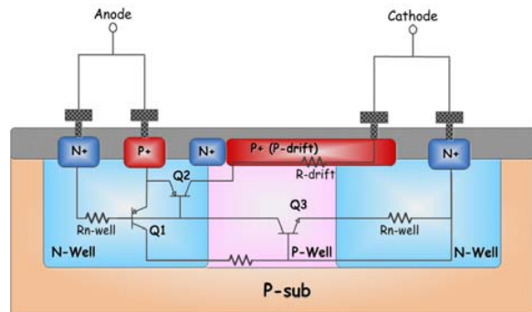
Fig. 3 A cross-sectional view of ZTSCR (Zener Triggering SCR)
