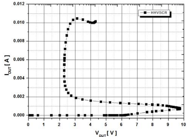
Fig. 7 I-V Characteristics curve of the HHVSCR
