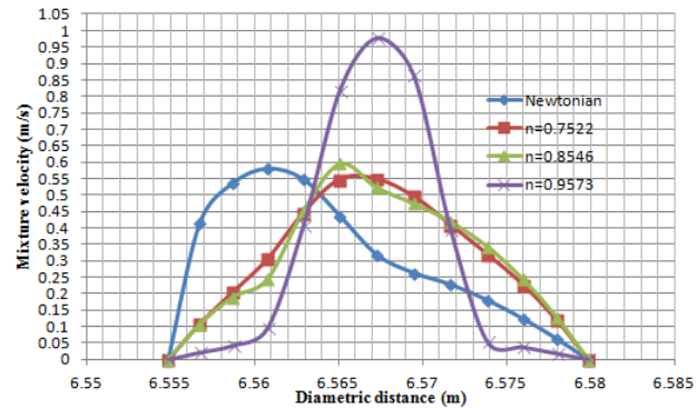
Fig. 8 Diametric distribution of mixture velocity at different flow behavior index
