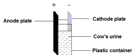
Fig. 2 Schematic representation of a single bio-voltaic cell
