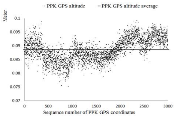
Fig. 9 Accuracies of PPK GPS altitude
