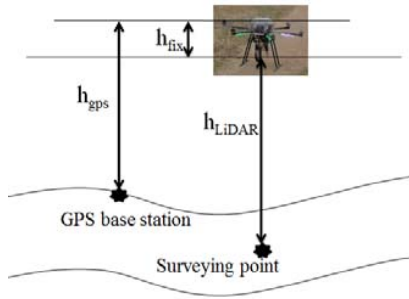
Fig. 7 Illustration of calculating ground height of each surveying point
