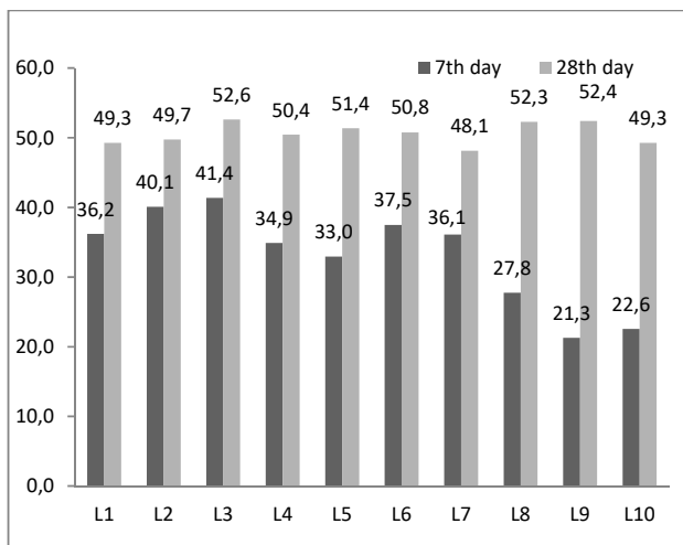
Fig. 4 Compressive Strength of Latex Series
