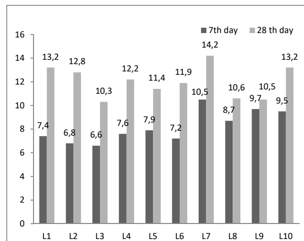
Fig. 2 Flexural Strength of Latex Series
