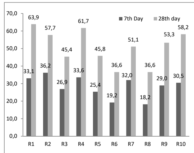
Fig. 5 Compressive Strength of RDP Series
