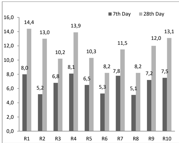
Fig. 3 Flexural Strength of RDP Series
