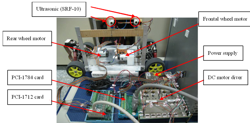
Fig. 1 Model vehicle structure and control circuit
