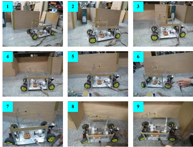
Fig. 7 Nine instantaneous motion pictures of vehicle roadside parallel auto-parking operation with SOFC control
