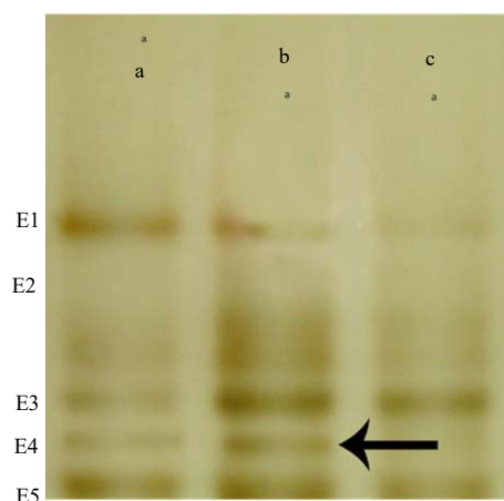
Fig. 1 Native PAGE profile of esterase isozyme from the workers of different population of Pasmmotermes hypostoma (a) Dar El-Salaam, (b) Qena and (c) El-Kawther
