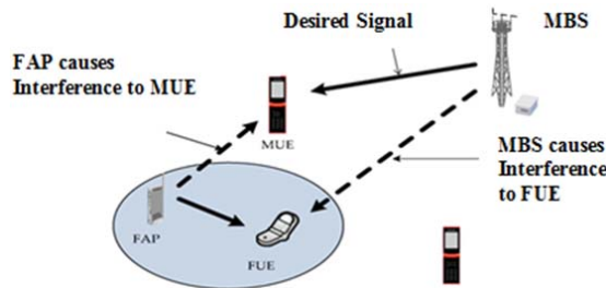
Fig. 3 Cross tier inter-cellular interference
