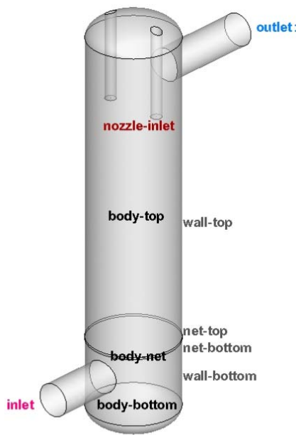
Fig. 2 Liquid nitrogen spray heat exchanger model
