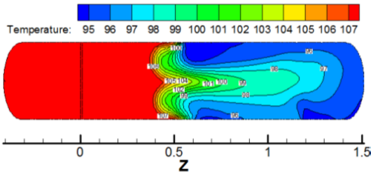
Fig. 9 The temperature contour (X=0)
