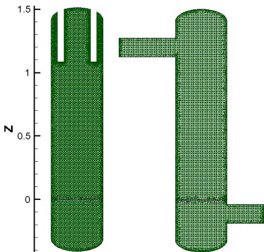
Fig. 4 Heat exchanger x = 0, y = 0 section grid
