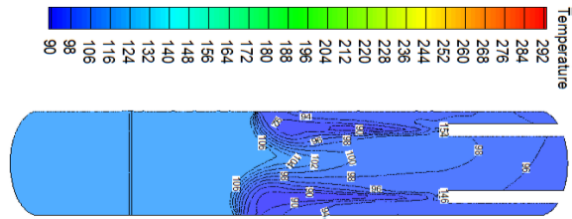
Fig. 11 The temperature contour (nozzle section)
