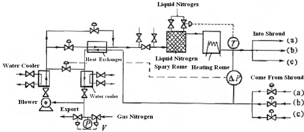
Fig. 1 Gas nitrogen thermostat equipment flow chart
